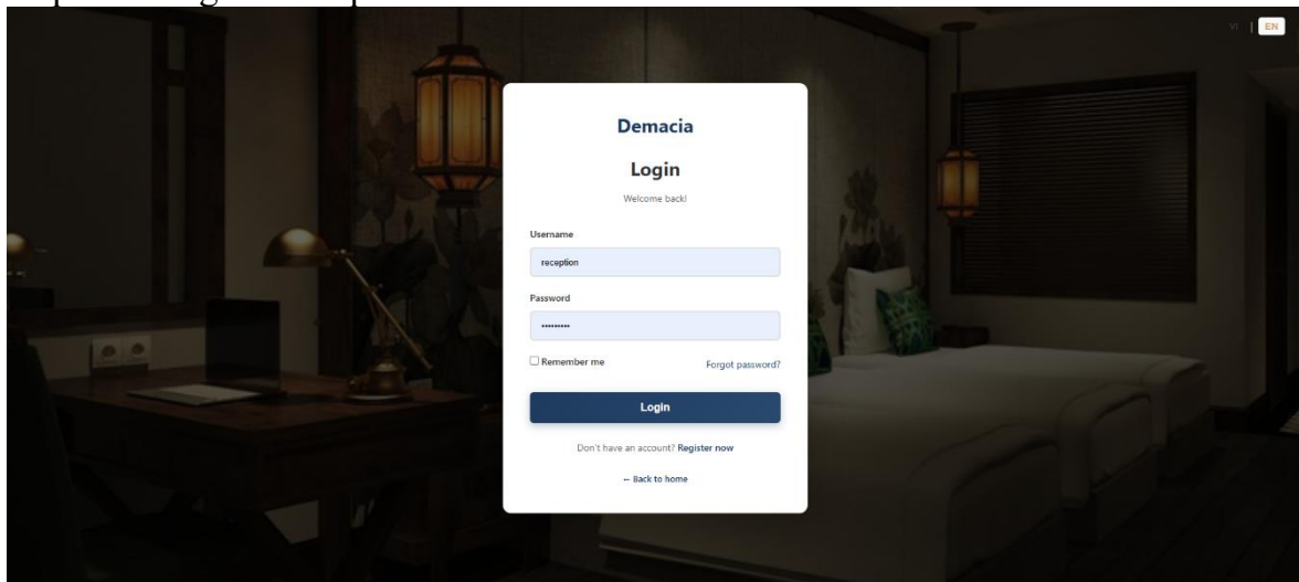
Figure 14: Login
